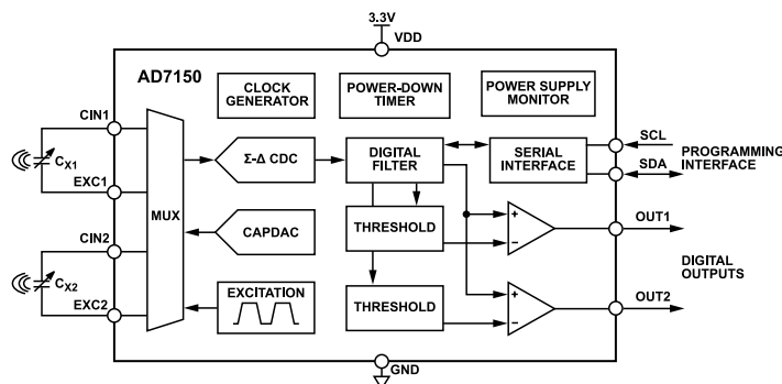
Figure 22. AD7150 Block Diagram
