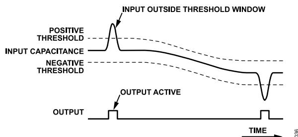
Figure 28. Out-Window (Adaptive) Threshold Mode
