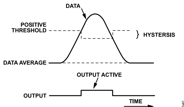
Figure 32. Threshold Hysteresis
