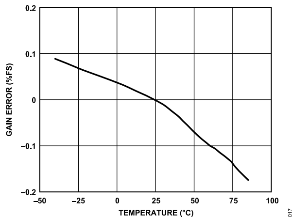
Figure 17. Capacitance Input Gain Error vs. Temperature, V_{DD} = 3.3\text{ V} , C_{IN} to EXC = 2\text{ pF}
