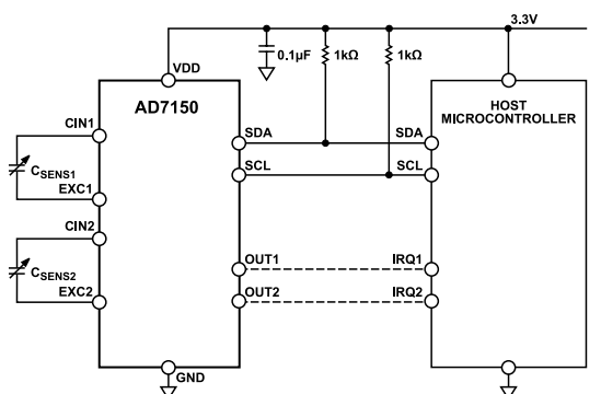
Figure 52. AD7150 Interfaced to a Host Microcontroller
