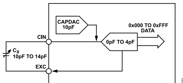
Figure 24. Using CAPDAC
