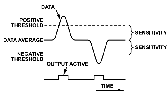
Figure 37. Threshold Sensitivity
