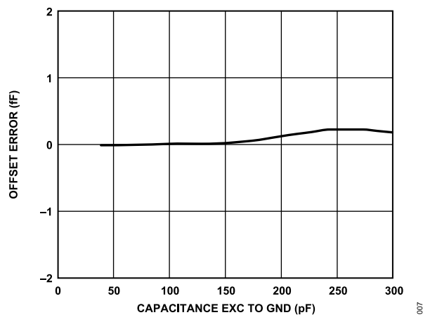
Figure 7. Capacitance Input Offset Error vs. Capacitance C_{EXC} to GND, V_{DD} = 3.3 V, C_{IN} Pin Open Circuit
