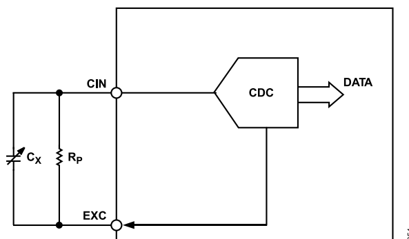
Figure 46. Parasitic Parallel Resistance
