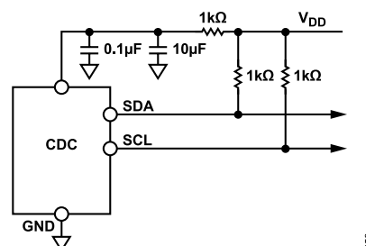
Figure 50. AD7150 V_{DD} Decoupling and Filtering
