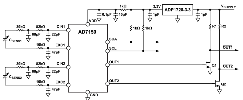
Figure 53. AD7150 Standalone Operation with EMC Protection
