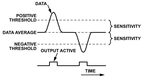
Figure 31. Threshold Sensitivity
