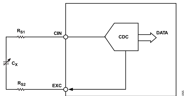
Figure 47. Parasitic Serial Resistance
