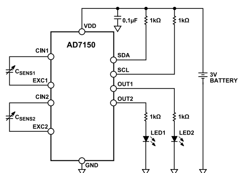
Figure 51. AD7150 Standalone Operation Application Diagram
