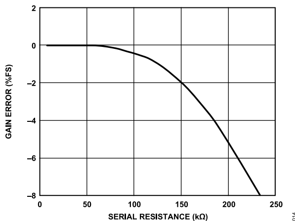
Figure 14. Capacitance Input Gain Error vs. Serial Resistance, V_{DD} = 3.3 V, C_{IN} to EXC = 2 pF
