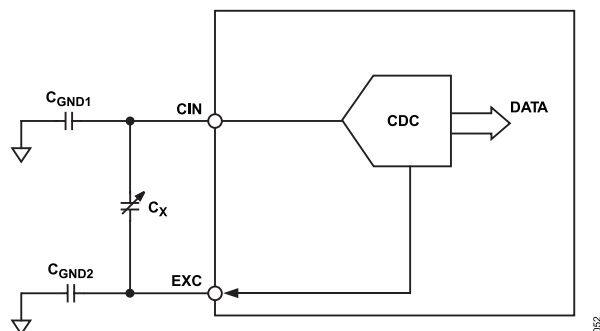
Figure 44. Parasitic Capacitance to Ground
