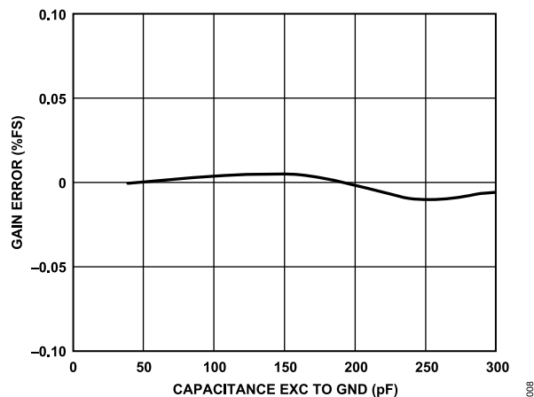
Figure 8. Capacitance Input Gain Error vs. Capacitance C_{EXC} to GND, V_{DD} = 3.3 V, C_{IN} to EXC = 2 pF
