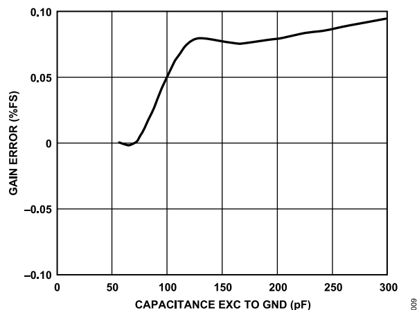
Figure 9. Capacitance Input Gain Error vs. Capacitance C_{EXC} to GND, V_{DD} = 3.3 V, C_{IN} to EXC = 10 pF
