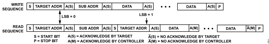
Figure 43. Write and Read Sequences
