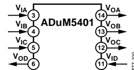
Figure 2. ADuM5401
