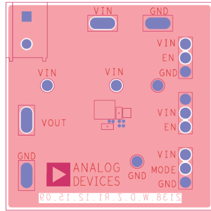
Figure 38. Bottom Layer
