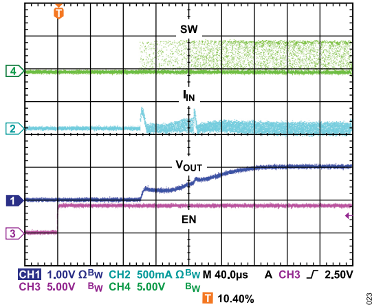
Figure 27. Startup, V_{OUT} = 0.8\text{ V} , I_{OUT} = 10\text{ mA}
