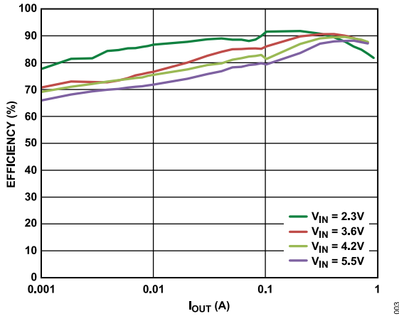
Figure 3. Efficiency vs. Load Current, Across Input Voltage, V_{OUT} = 1.8\text{ V} , PSM Mode
