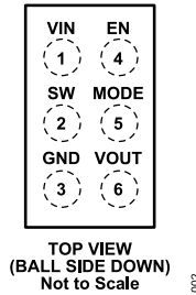
Figure 2. Pin Configuration (Top View)
