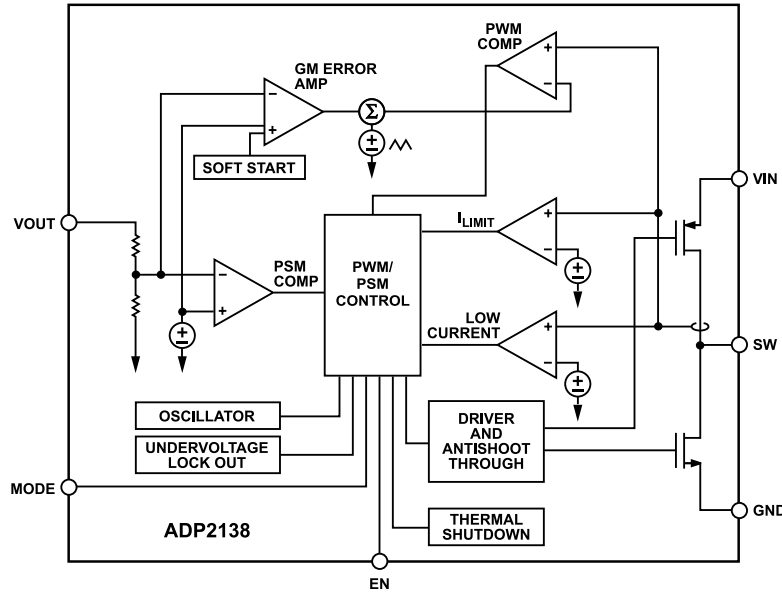
Figure 33. ADP2138 Functional Block Diagram
