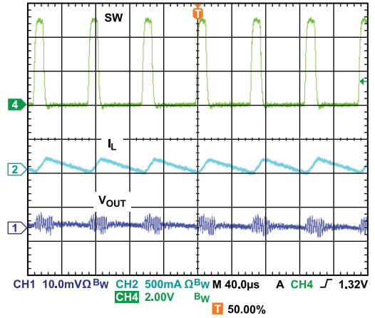
Figure 30. Typical Waveform, V_{OUT} = 1.8\text{ V} , PWM Mode, I_{OUT} = 200\text{ mA}
