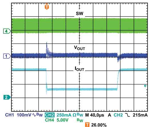
Figure 19. Response to Load Transient, 150 mA to 500 mA, V_{OUT} = 0.8 V, PWM Mode
