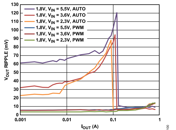
Figure 32. V_{OUT} Peak-to-Peak Ripple vs. Output Current, V_{OUT} = 1.8\text{ V}
