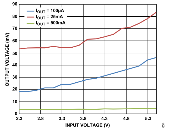
Figure 14. Output Voltage Ripple vs. Input Voltage, Across Output Current, V_{OUT} = 1.8\text{ V}
