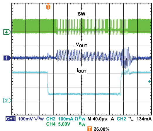
Figure 20. Response to Load Transient, 50 mA to 200 mA, V_{OUT} = 0.8 V, Automatic Mode
