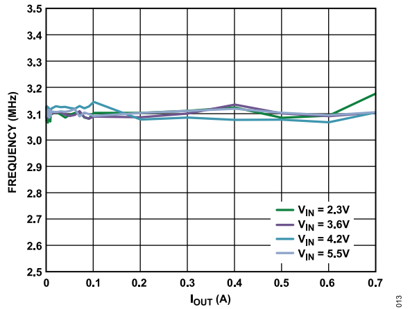
Figure 13. Frequency vs. Output Current, Across Supply Voltage, V_{OUT} = 1.8\text{ V}
