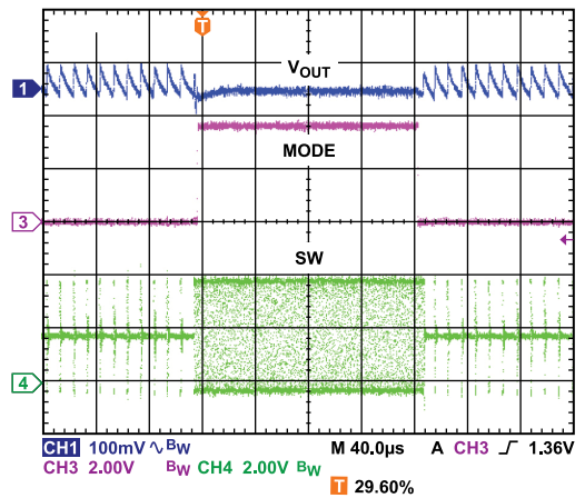
Figure 31. Mode Transition from PSM to PWM to PSM, V_{OUT} = 1.8\text{ V}
