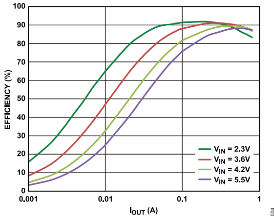
Figure 4. Efficiency vs. Load Current, Across Input Voltage, V_{OUT} = 1.8\text{ V} , PWM Mode
