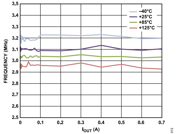
Figure 12. Frequency vs. Output Current, Across Temperature, V_{OUT} = 1.8\text{ V} , PWM Mode
