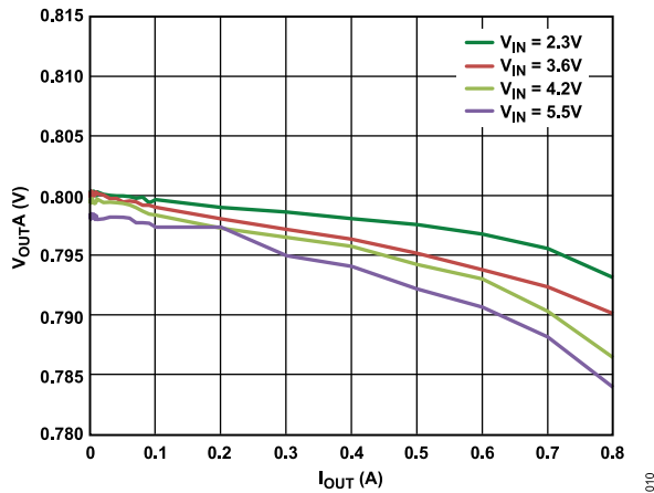
Figure 10. Load Regulation Across Input Voltage, V_{OUT} = 0.8\text{ V} , PWM Mode
