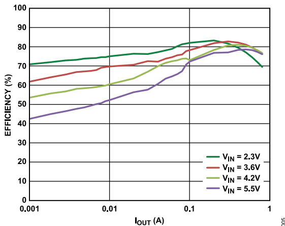
Figure 5. Efficiency vs. Load Current, Across Input Voltage, V_{OUT} = 0.8\text{ V} , PSM Mode
