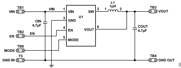
Figure 36. Evaluation Board Schematic
