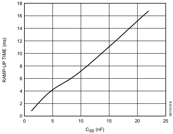
Figure 19. Output Voltage Ramp-Up vs. Soft-Start Capacitor Value
