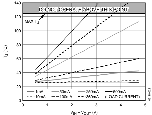
Figure 34. 700 mm 2 PCB Copper, T A = 25°C
