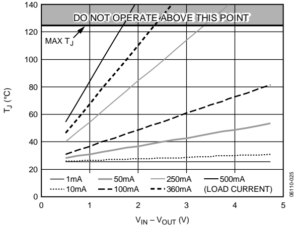
Figure 37. 0 mF of PCB Copper, \pm 25^{\circ}\text{C}
