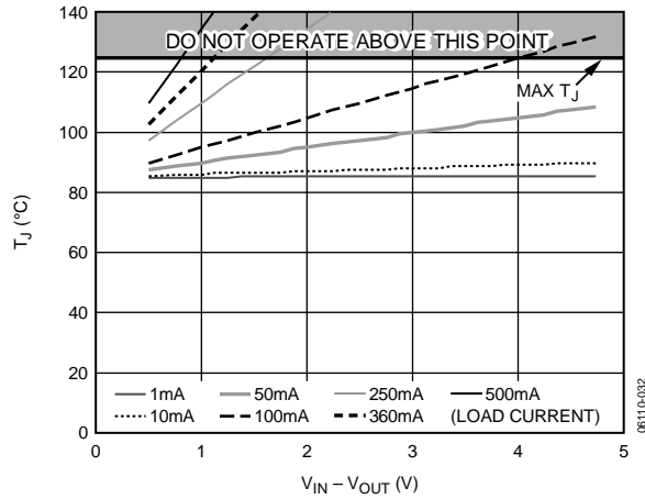
Figure 44. 100 m 2 of PCB Copper, \pm 85^{\circ}\text{C}
