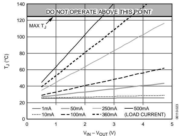
Figure 35. 300 mm 2 PCB Copper, T A = 25°C
