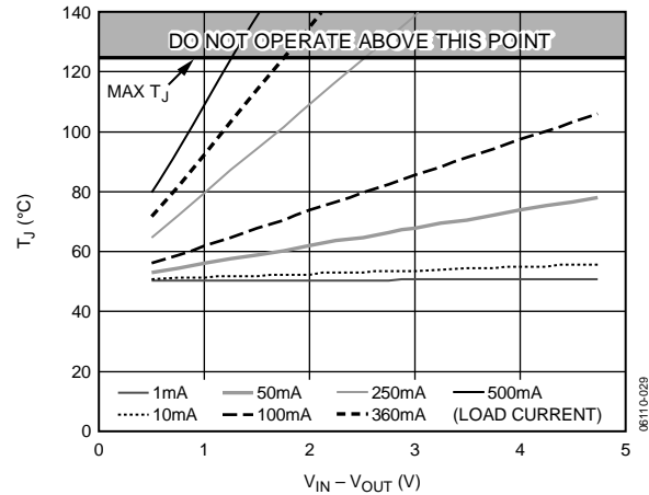
Figure 41. 0 mF of PCB Copper, \pm 50^{\circ}\text{C}
