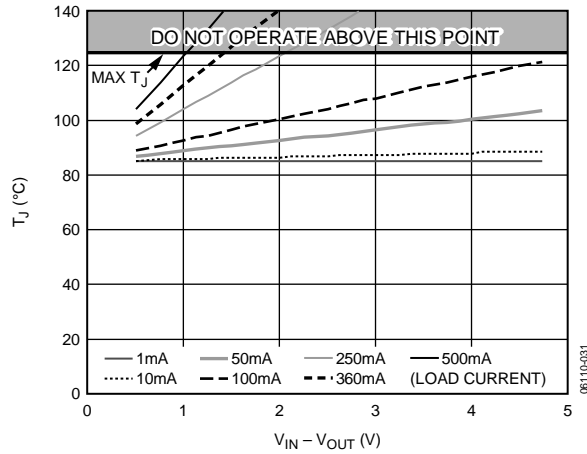
Figure 43. 300 m 2 of PCB Copper, \pm 85^{\circ}\text{C}
