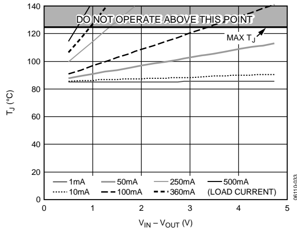
Figure 45. 0 m 2 of PCB Copper, \pm 85^{\circ}\text{C}
