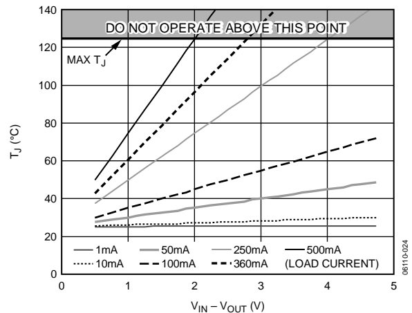
Figure 36. 100 mm 2 PCB Copper, T A = 25°C
