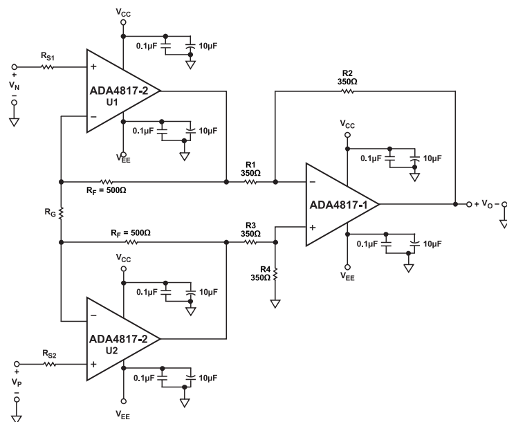
Figure 66. High Speed Instrumentation Amplifier
