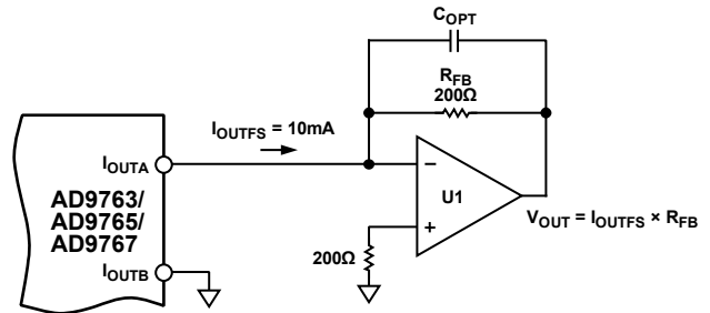
Figure 76. Unipolar Buffered Voltage Output
