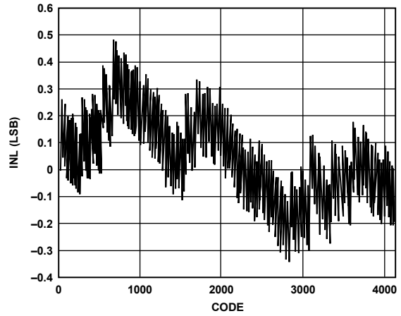
Figure 33. Typical INL
