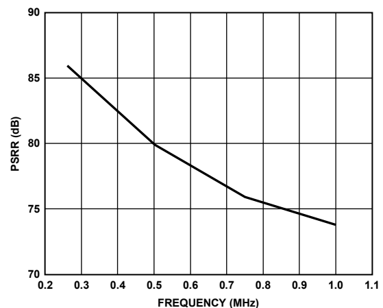
Figure 77. AVDD Power Supply Rejection Ratio vs. Frequency
