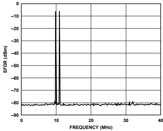
Figure 21. Dual-Tone SFDR @ f_{CLK} = 125 \text{ MSPS}
