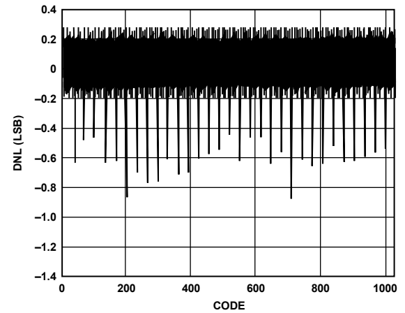
Figure 51. Typical DNL
