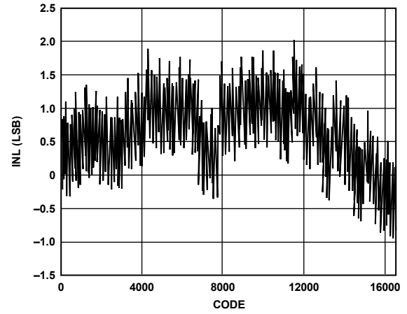
Figure 50. Typical INL
