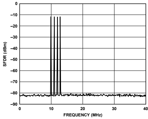
Figure 22. Four-Tone SFDR @ f_{CLK} = 125 \text{ MSPS}
