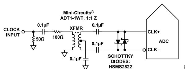
Figure 61. Transformer-Coupled Differential Clock (Up to 200 MHz)
