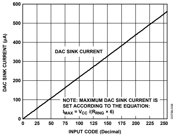
Figure 25. DAC Sink Current vs. Input Code with R_{RING} = 1k
