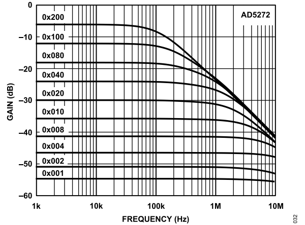
Figure 27. 50 kΩ Gain vs. Code vs. Frequency
