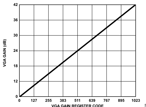
Figure 38. VGA Gain Curve (PxGA Not Included)
