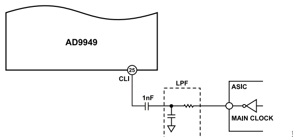
Figure 43. CLI Connection, AC-Coupled
