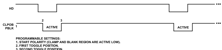
Figure 22. Clamp and Preblank Pulse Placement
