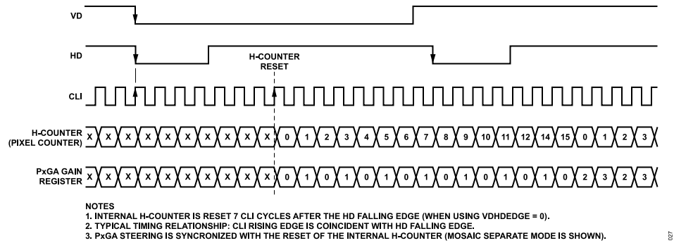
Figure 27. H-Counter Synchronization
