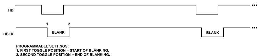
Figure 23. Horizontal Blanking (HBLK) Pulse Placement
