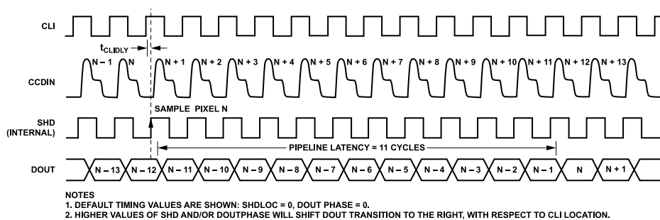
Figure 21. Pipeline Delay for Digital Data Output
