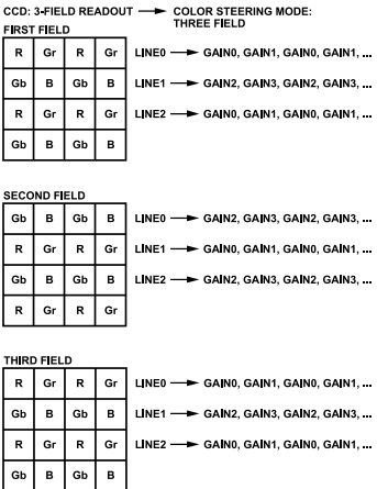
Figure 33. CCD Color Filter Example—Three-Field Readout
