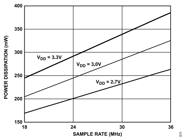
Figure 11. Power Curves
