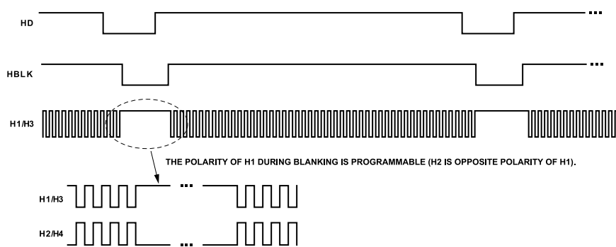
Figure 24. HBLK Masking Control
