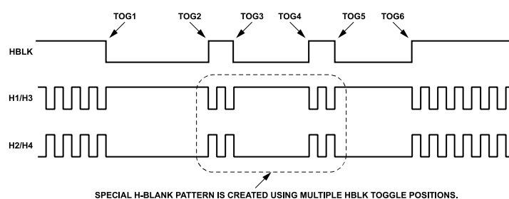
Figure 25. Generating Special HBLK Patterns
