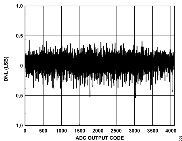
Figure 9. Typical DNL
