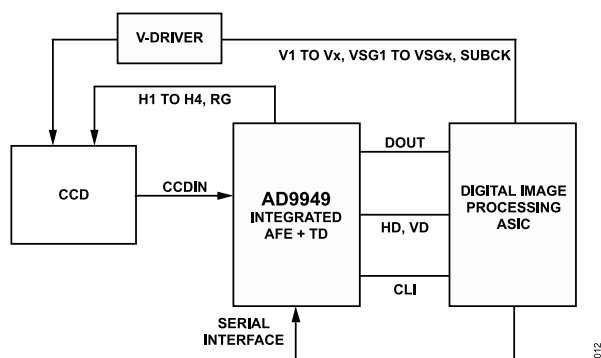
Figure 12. Typical Application
