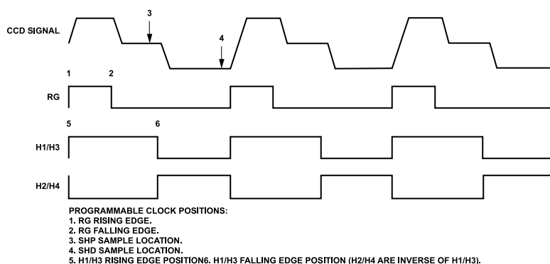
Figure 18. High Speed Clock Programmable Locations
