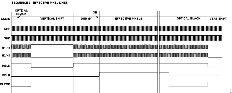
Figure 47. Horizontal Sequences During Effective Pixels
