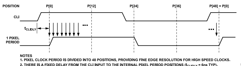
Figure 17. High Speed Clock Resolution from CLI Main Clock Input
