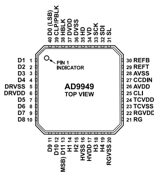
Figure 3. Pin Configuration
