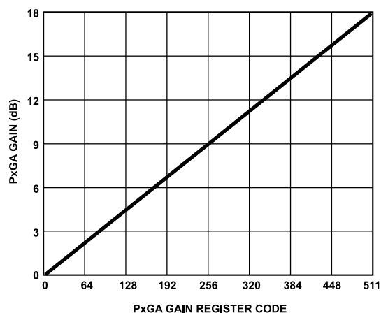
Figure 37. PxGA Gain Curve
