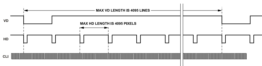
Figure 14. Maximum VD/HD Dimensions
