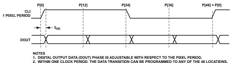
Figure 20. Digital Output Phase Adjustment
