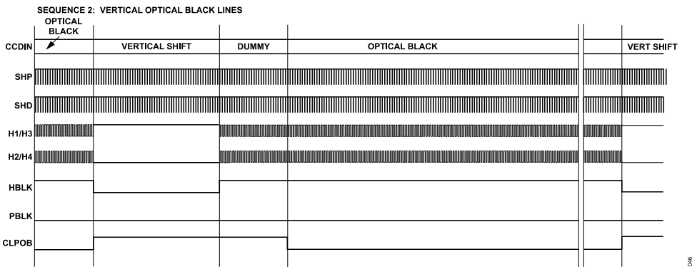
Figure 46. Horizontal Sequences During Vertical Optical Black Pixels
