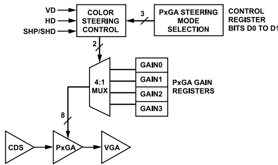
Figure 30. PxGA Block Diagram
