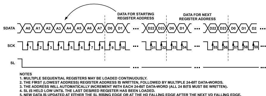
Figure 16. Continuous Serial Write Operation
