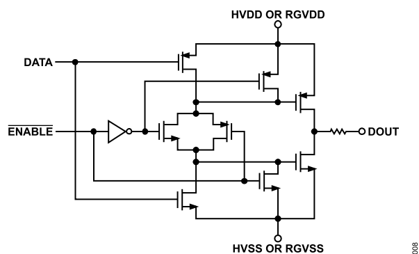
Figure 8. H1 to H4 and RG (Pins 14 to 15, 18 to 19, 21)
