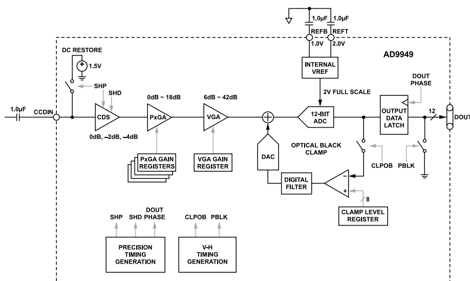
Figure 29. Analog Front End Functional Block Diagram
