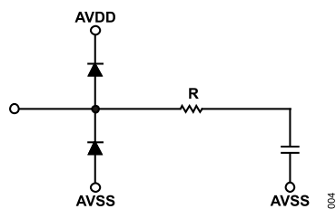
Figure 4. CCDIN (Pin 27)
