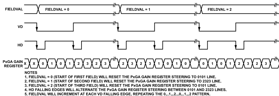
Figure 36. PxGA Color Steering—Three-Field Mode
