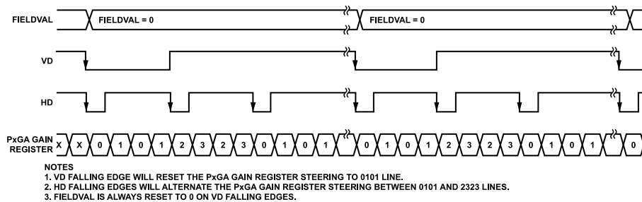
Figure 34. PxGA Color Steering—Progressive Mode
