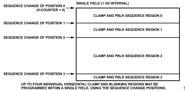
Figure 26. Clamp and Blanking Sequence Flexibility
