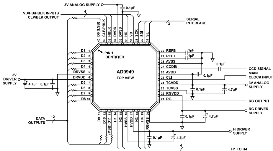
Figure 39. Recommended Circuit Configuration
