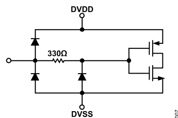
Figure 7. Digital Inputs (Pins 31 to 35, 38)
