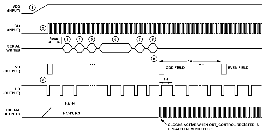
Figure 28. Recommended Power-Up Sequence
