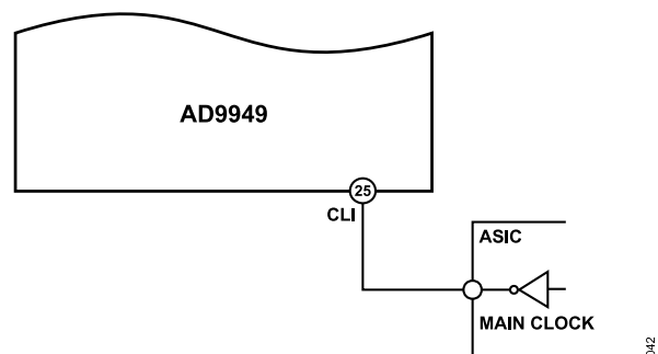
Figure 42. CLI Connection, DC-Coupled
