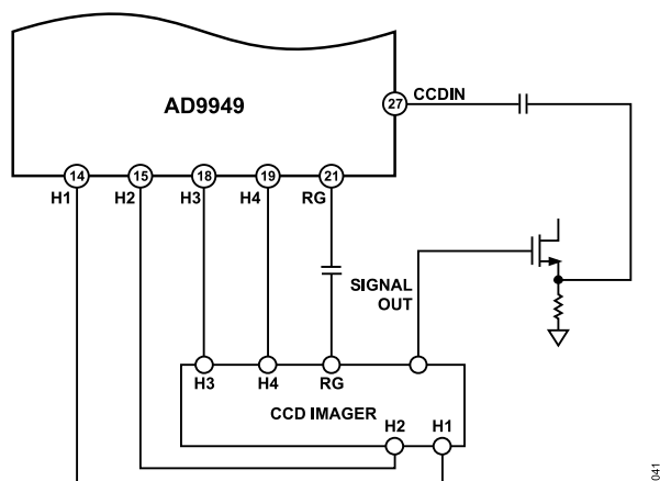
Figure 41. CCD Connections (4 H-Clock)
