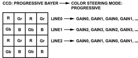
Figure 31. CCD Color Filter Example—Progressive Scan
