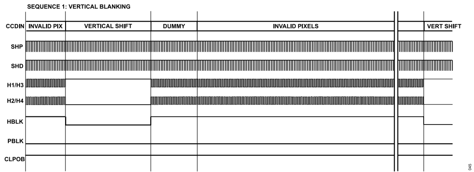
Figure 45. Horizontal Sequence During Vertical Blanking
