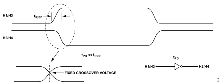
Figure 19. H-Clock Inverse Phase Relationship
