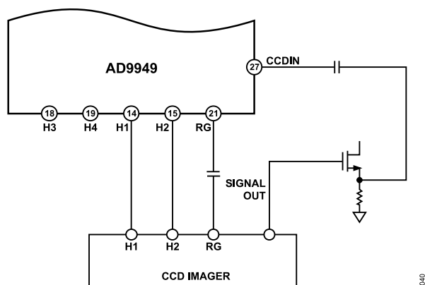
Figure 40. CCD Connections (2 H-Clock)
