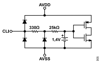
Figure 5. CLI (Pin 25)
