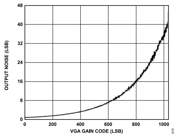
Figure 10. Output Noise vs. VGA Gain
