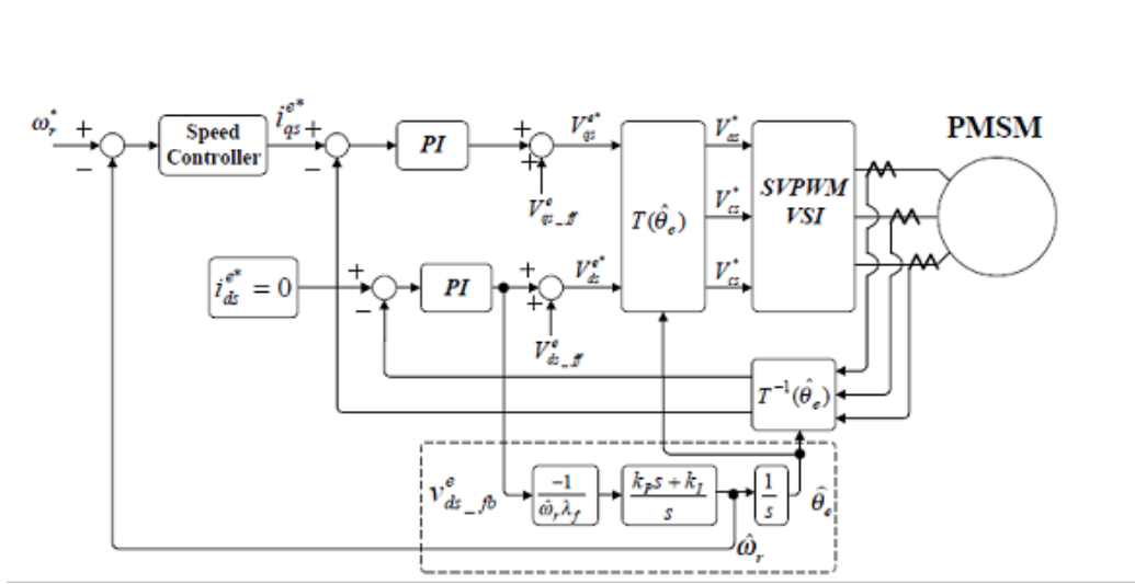
Figure 1. Balance of Back EMF and initial start (attributed to Bon-Ho Bae)
