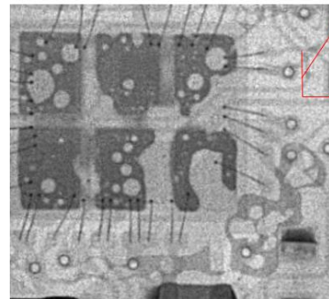
Solder flow under die
