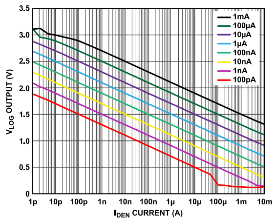
Figure 9. V_{LOG} vs. I_{DEN} for Multiple Values of I_{NUM} (Decade Steps from 100 pA to 1 mA)
