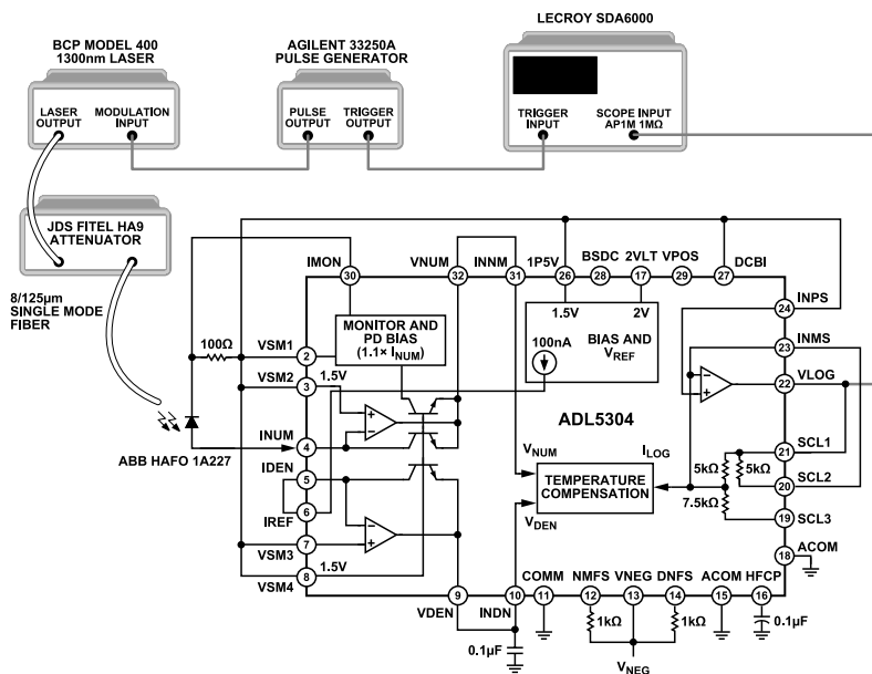
Figure 41. Setup for Measuring Photodiode Pulse Response
