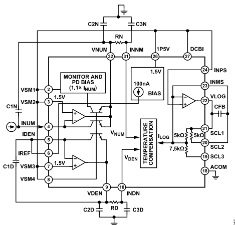
Figure 48. Possible External Filtering Locations
