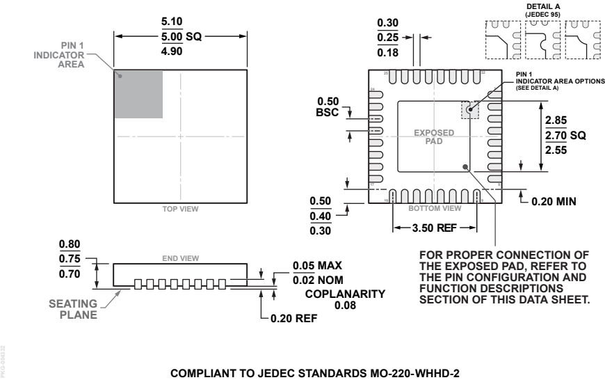
Figure 61. 32-Lead Lead Frame Chip Scale Package [LFCSP] 5 mm × 5 mm Body and 0.75 mm Package Height (CP-32-21) Dimensions shown in millimeters
