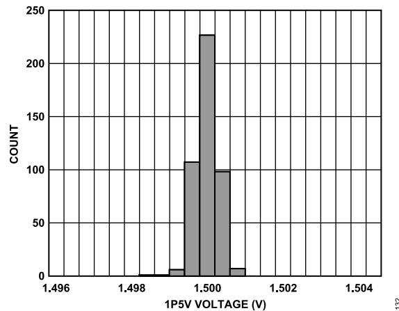
Figure 32. 1P5V Histogram
