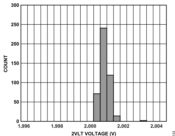
Figure 33. 2VLT Histogram
