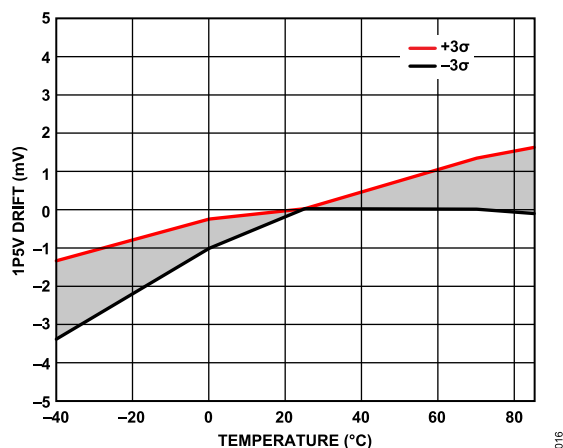
Figure 16. 1P5V Drift vs. Temperature
