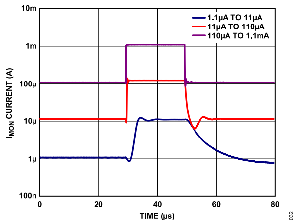
Figure 28. I_{MON} Pulse Response vs. I_{NUM}
