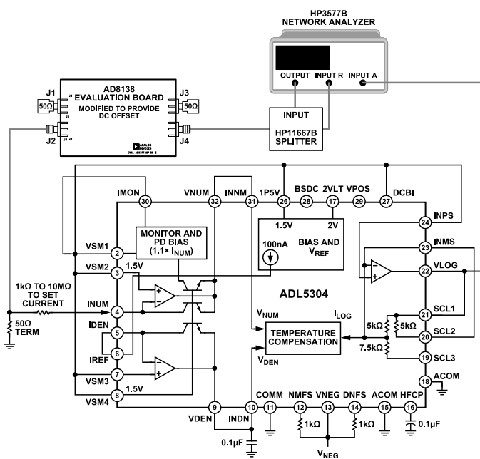
Figure 39. Setup for Measuring Bandwidth
