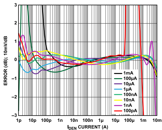
Figure 12. Law Conformance Error vs. I_{DEN} for Multiple Values of I_{NUM} (Decade Steps from 100 pA to 1 mA)
