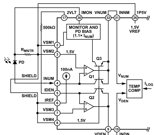
Figure 52. Intercept Shifted One Decade Right via External Resistor, Reference Current I_{DEN} = 1 \mu A
