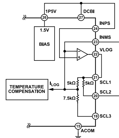
Figure 51. Buffer Amplifier in Default Configuration
