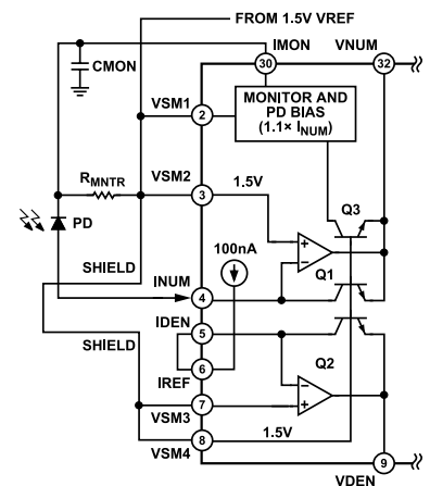
Figure 49. Adaptive Photodiode Bias
