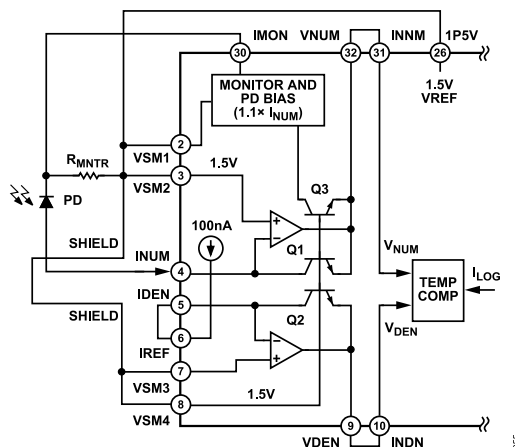
Figure 45. Simplified Front-End Schematic
