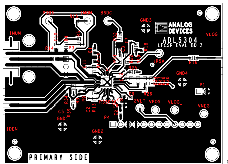
Figure 59. Evaluation Board, Primary Side
