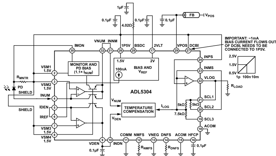
Figure 55. Basic Connections for Single-Supply Operation
