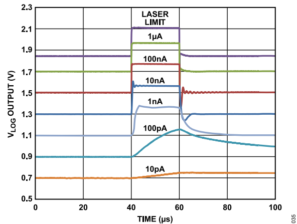
Figure 56. Photodiode Response for Input Currents of Approximately 10 pA to >1 \mu A Where Laser Limit Encountered
