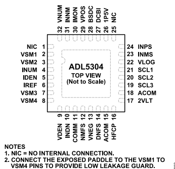
Figure 2. 32-Lead LFCSP Pin Configuration
