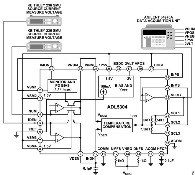
Figure 38. Setup for Measuring Logarithmic/Slope/Offset Conformance
