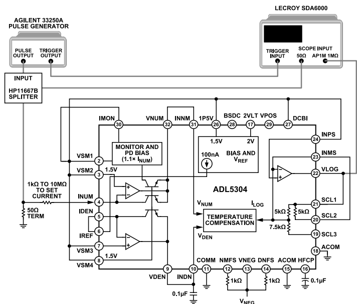
Figure 40. Setup for Measuring Pulse Settling
