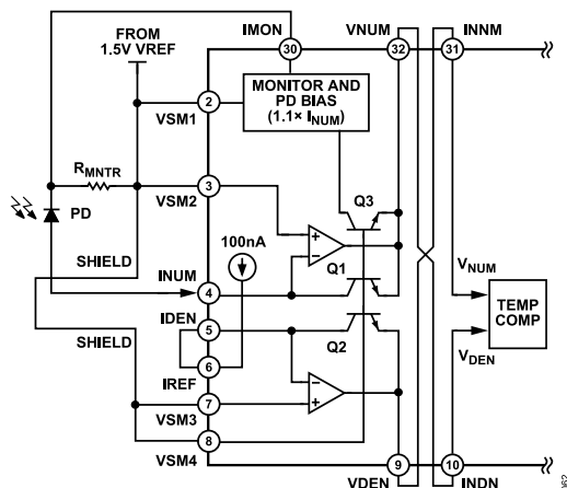
Figure 53. Simple Slope Inversion Method
