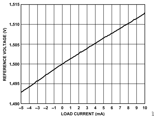
Figure 17. 1P5V vs. I_{LOAD} (Positive Current Defined into 1P5V Pin)
