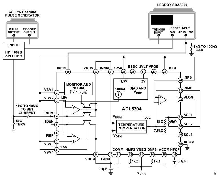
Figure 43. Setup for Measuring IMON Pulse Response
