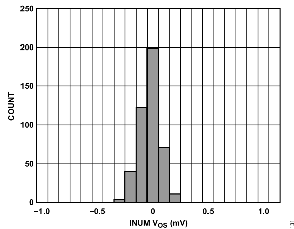
Figure 31. (V_{NUM} - V_{SUM}) Histogram at 25°C
