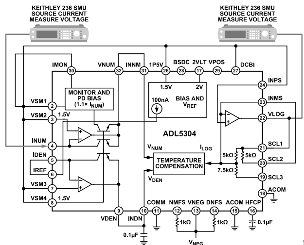
Figure 42. Setup for Measuring Output
