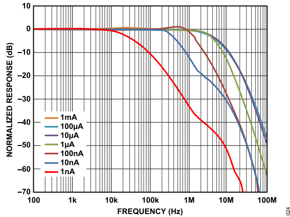
Figure 21. Small Signal AC Response from I_{NUM} to V_{LOG} for I_{NUM} in Decade Steps from 1 nA to 1 mA, I_{DEN} = 100 nA
