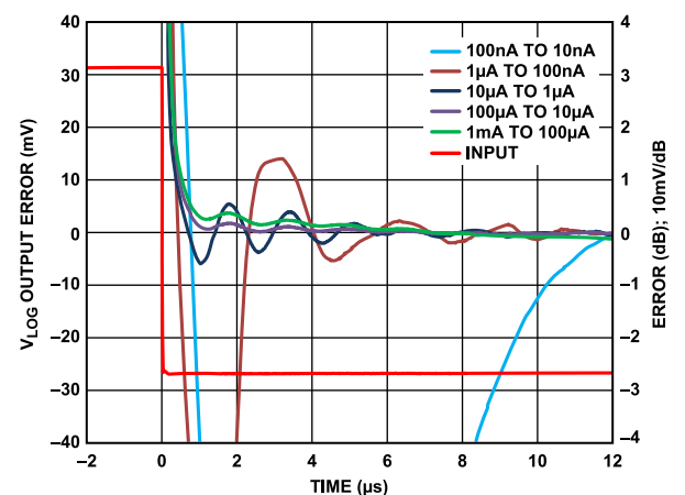
Figure 26. Normalized Falling Edge Settling of I_{NUM} to Within 1 dB (Error = 10 mV/dB)
