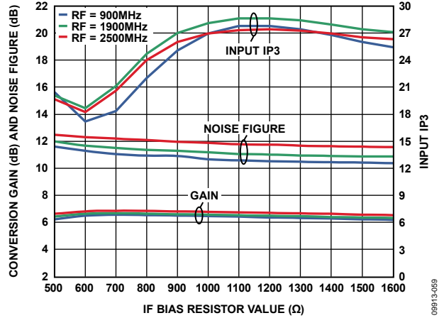
Figure 43. Power Conversion Gain, Noise Figure, and Input IP3 vs. IF Bias Resistor Value
