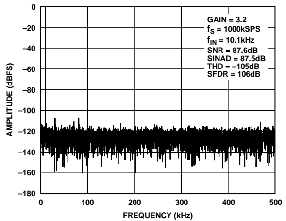
Figure 23. 10 kHz FFT, PGIA Gain = 3.2
