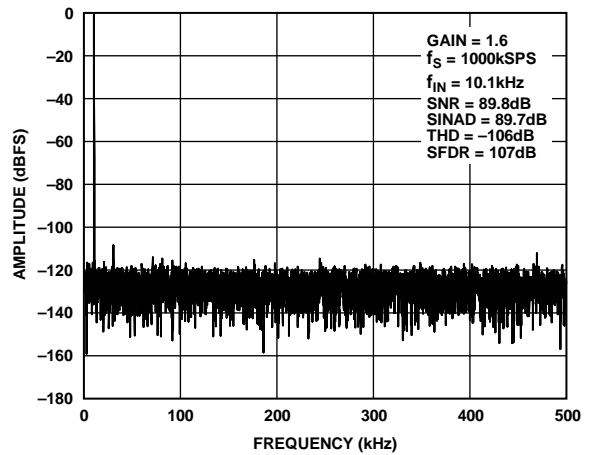
Figure 22. 10 kHz FFT, PGIA Gain = 1.6
