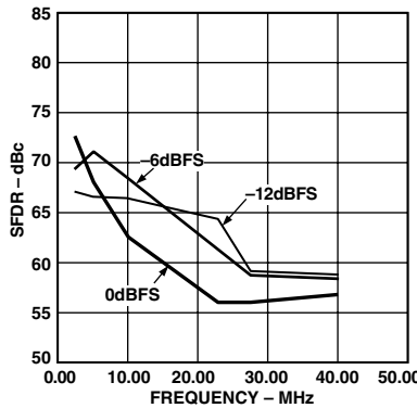
Figure 25. SFDR vs. f_{OUT} @ 100 MSPS
