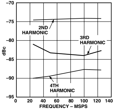
Figure 30. THD vs. f_{CLOCK} f_{OUT} = 2 \text{ MHz}
