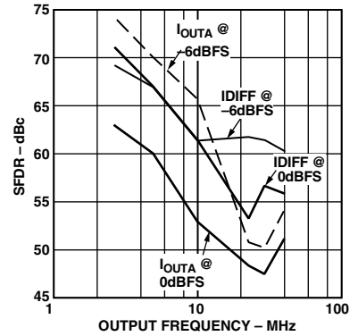
Figure 32. Differential vs. Single Ended SFDR vs. f_{OUT} @ 100 MSPS
