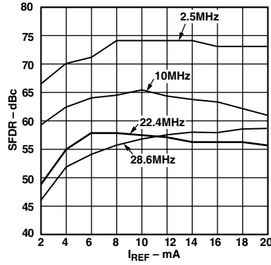
Figure 31. SFDR vs. f_{OUT} and I_{OUTFS} @ 100 MSPS, 0 dBFS
