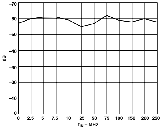
TPC 2. Crosstalk vs. f_{IN} : f_s = 140 MSPS
