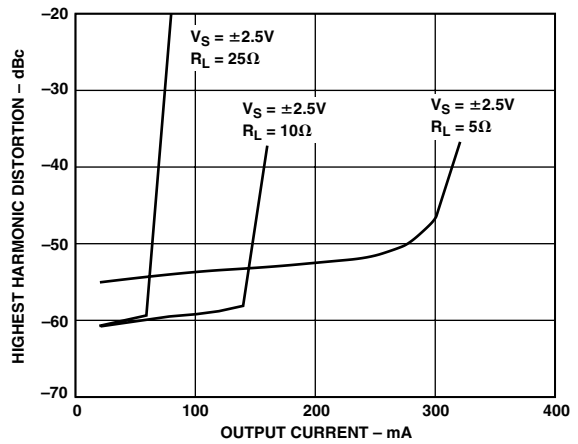
TPC 10. Distortion vs. Output Current; V_S = \pm 2.5\text{ V} , f = 1\text{ MHz} , G = +2
