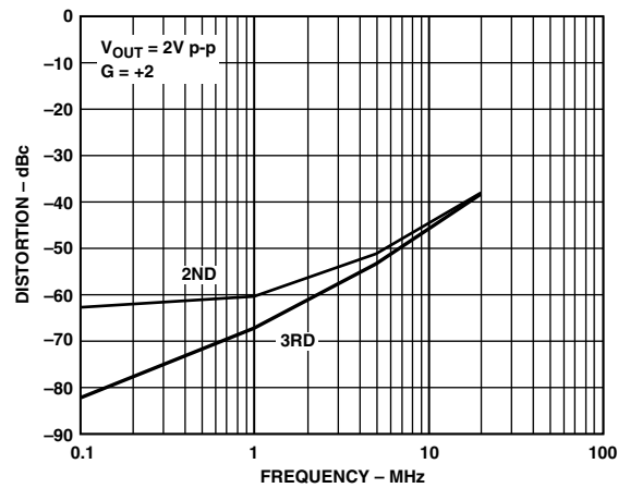
TPC 9. Distortion vs. Frequency; V_S = \pm 2.5\text{ V} , R_L = 25\ \Omega
