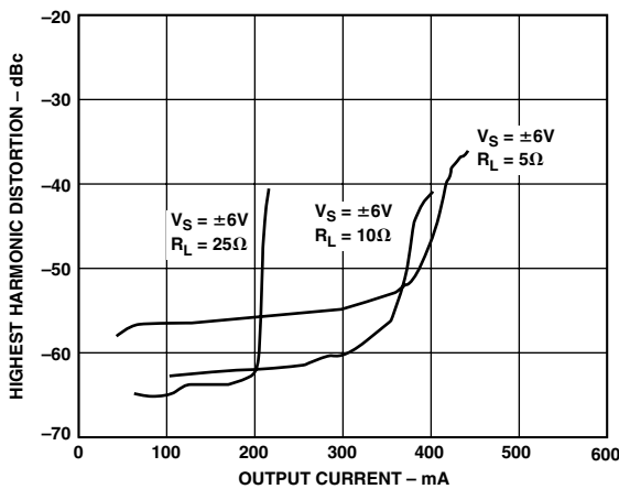
TPC 7. Distortion vs. Output Current; V_S = \pm 6\text{ V} , f = 1\text{ MHz} , G = +2
