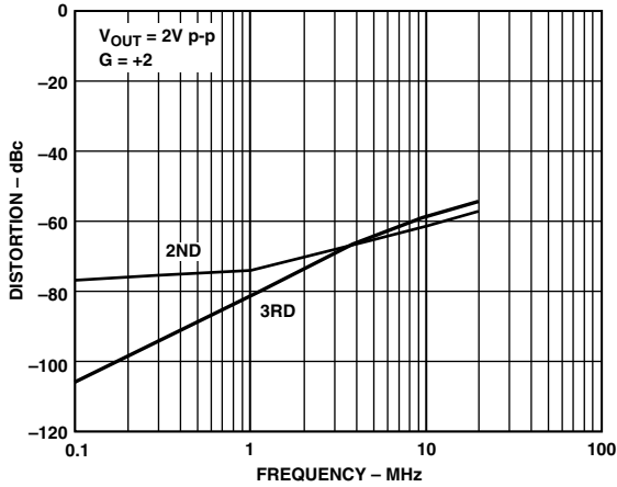
TPC 5. Distortion vs. Frequency; V_S = \pm 6\text{ V} , R_L = 100\ \Omega
