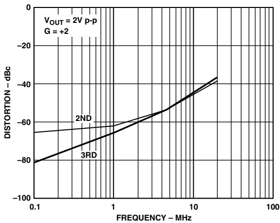
TPC 6. Distortion vs. Frequency; V_S = \pm 6\text{ V} , R_L = 25\ \Omega
