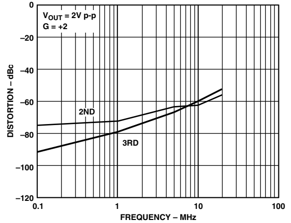
TPC 8. Distortion vs. Frequency; V_S = \pm 2.5\text{ V} , R_L = 100\ \Omega
