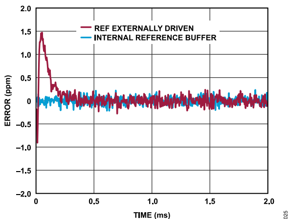
Figure 25. Error During Conversion Burst After Long Idle Time
