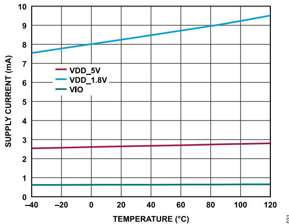
Figure 31. Supply Current vs. Temperature
