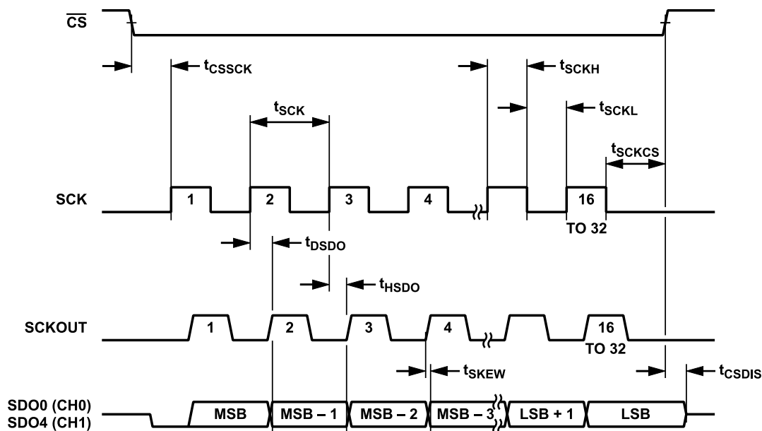
Figure 7. Echo Clock Mode Timing, SDR, 1-Lane
