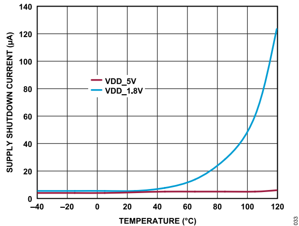
Figure 33. Supply Shutdown Current vs. Temperature
