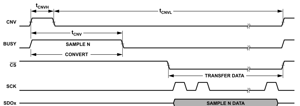
Figure 50. Basic Single Sample Conversion Cycle
