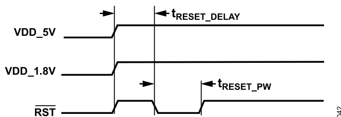
Figure 42. Power-On Reset (POR) Timing
