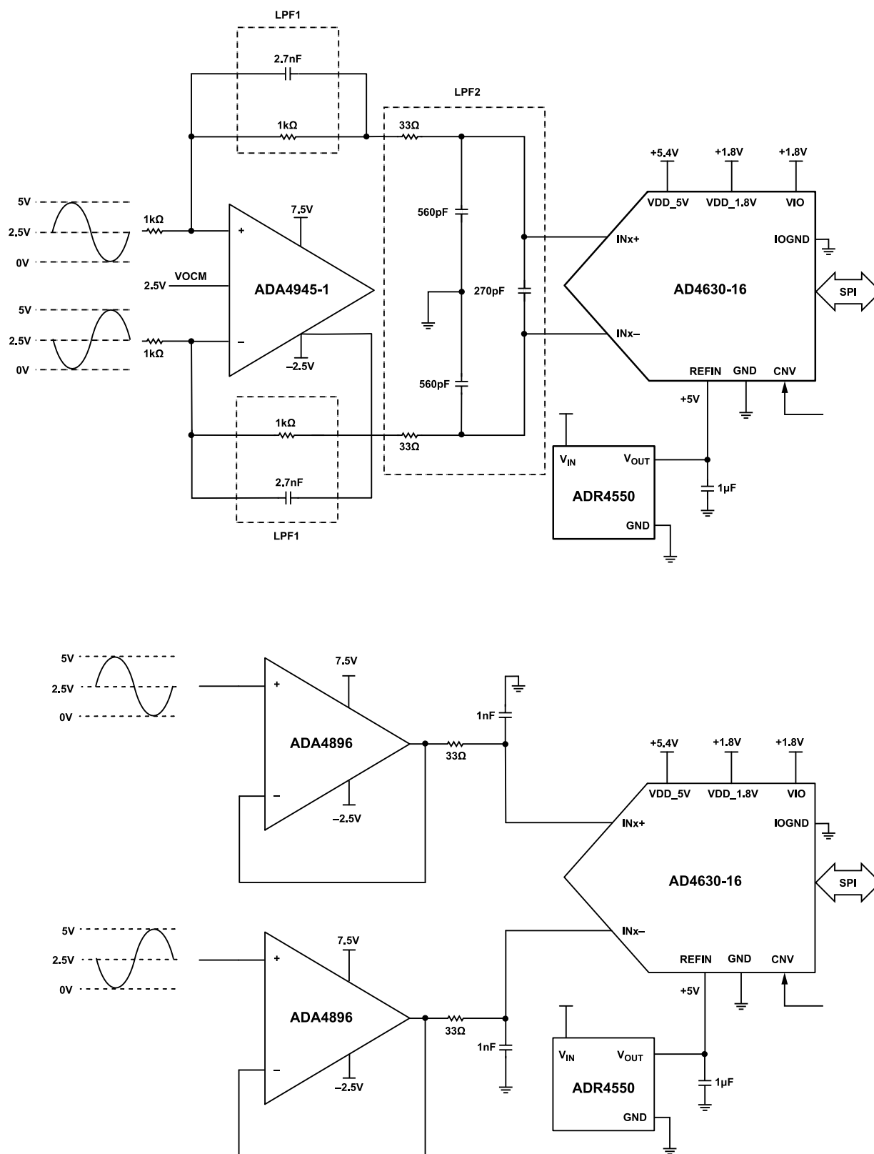
Figure 39. Typical Application Circuit Diagrams
