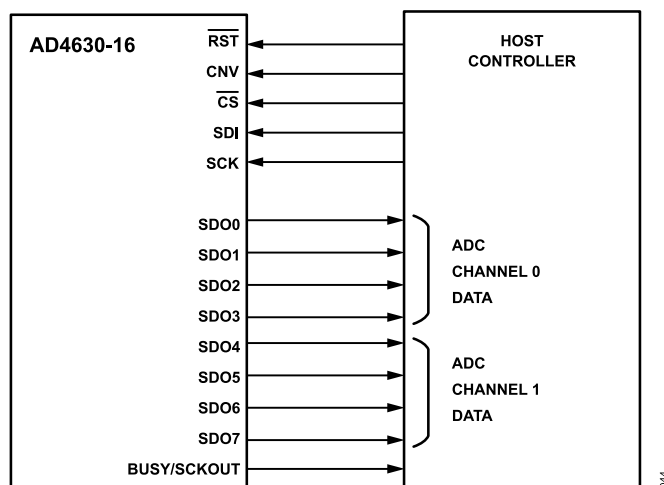
Figure 44. Multilane SPI
