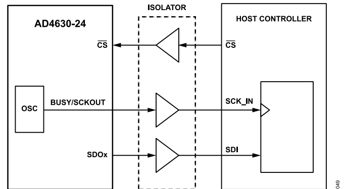
Figure 49. Host Clock Mode Signal Path Example
