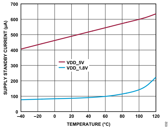
Figure 32. Supply Standby Current vs. Temperature
