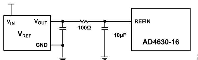
Figure 40. Reference with Noise Filter
