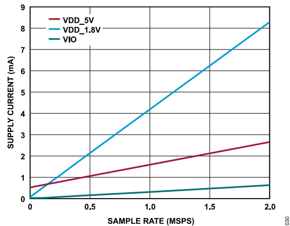
Figure 30. Supply Current vs. Sample Rate
