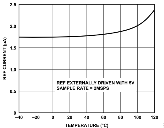
Figure 29. REF Current vs. Temperature
