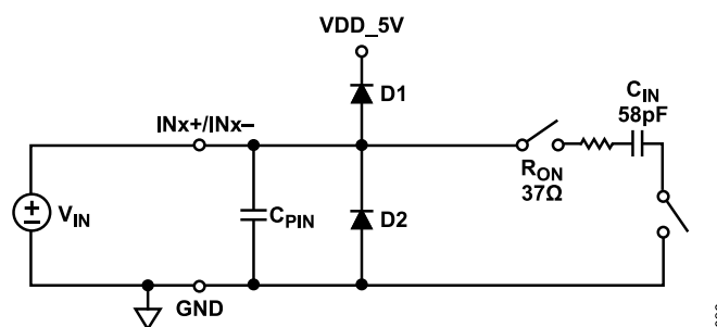
Figure 36. Equivalent Circuit for the AD4630-16 Differential Analog Input
