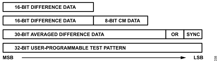
Figure 38. Summary of Selectable Output Sample Formats
