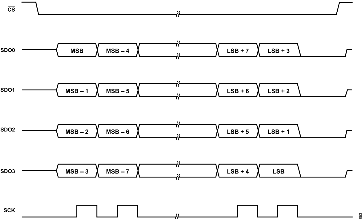
Figure 53. 4-Lane, SDR Timing Diagram
