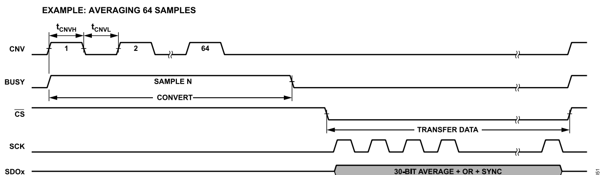
Figure 51. Example Conversion Cycle for Averaging Mode
