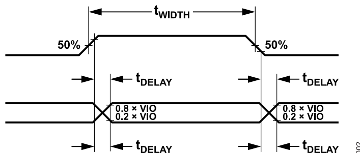
Figure 2. Voltage Levels for Timing
