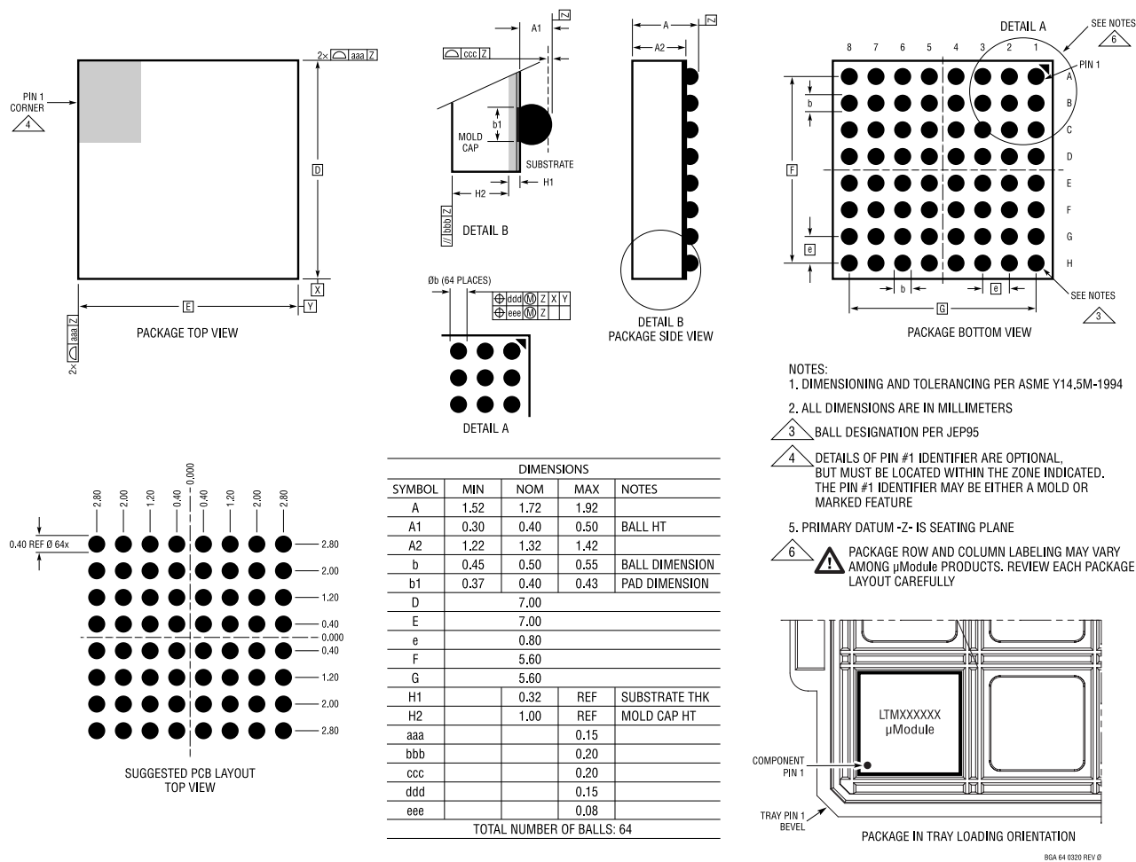
Figure 55. 64-Ball Chip Scale Package Ball Grid Array [CSP_BGA] (05-08-1797) Dimensions shown in millimeters
