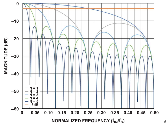
Figure 37. Frequency Response Examples for the Block Averaging Filter
