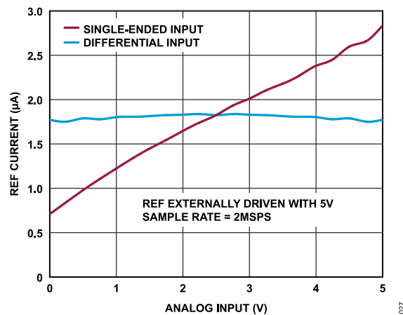
Figure 27. REF Current vs. Analog Input
