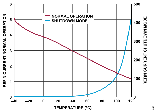
Figure 26. REFIN Current Normal Operation and REFIN Current Shutdown Mode vs. Temperature
