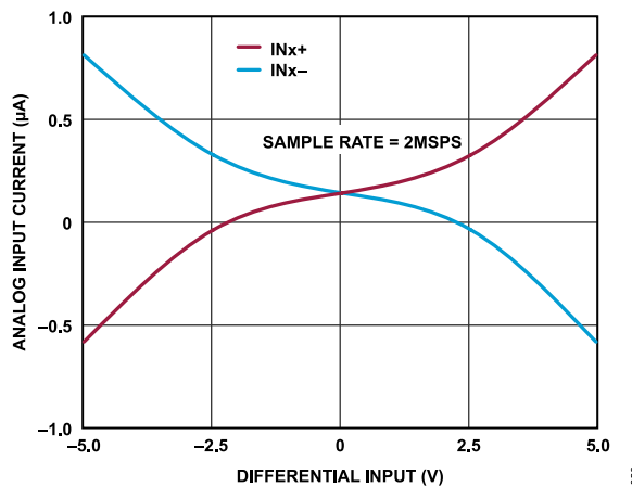
Figure 23. Analog Input Current vs. Differential Input
