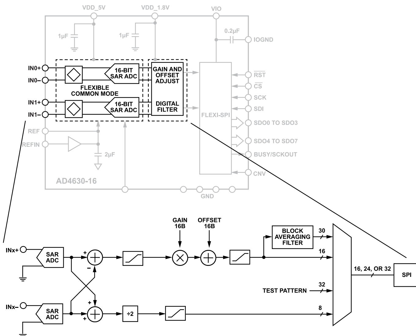
Figure 34. Functional Block Diagram and Channel Architecture
