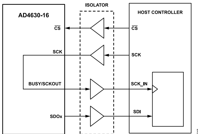
Figure 48. Echo Clock Mode Signal Path Diagram
