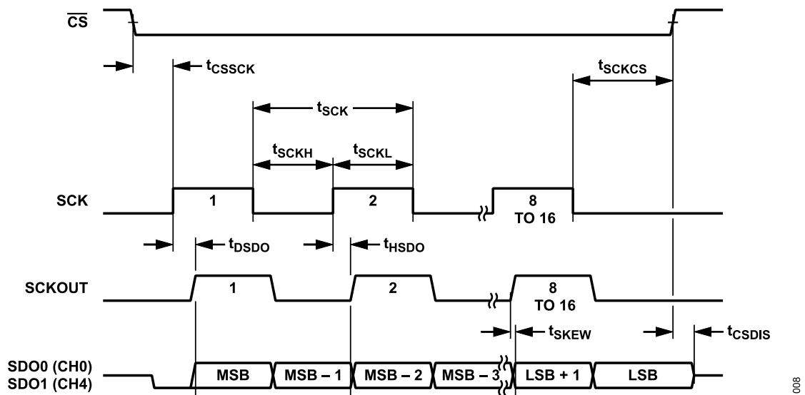
Figure 8. Echo Clock Mode Timing, DDR, 1-Lane
