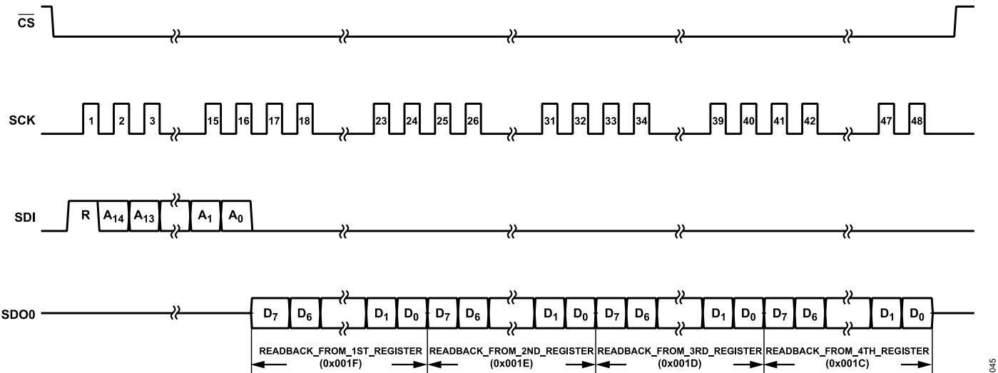
Figure 45. Stream Mode Bulk Register Read Back Operation
