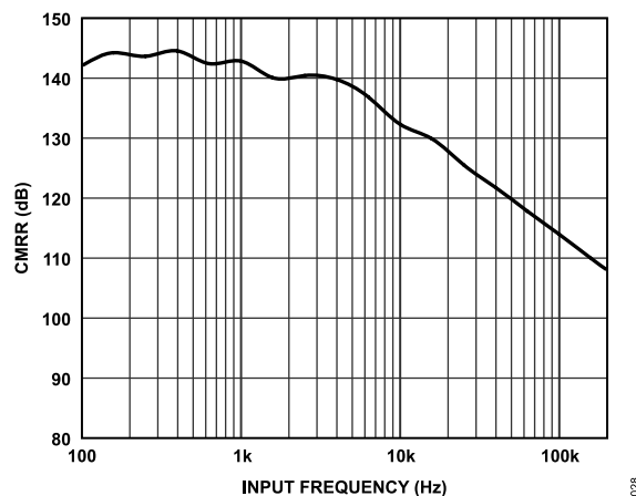
Figure 28. CMRR vs. Input Frequency
