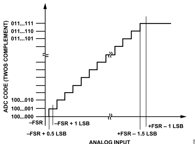
Figure 35. ADC Ideal Transfer Function for the Differential Output Codes (FSR Is Full-Scale Range)
