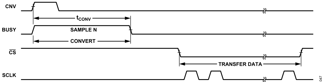
Figure 47. Typical Sample Cycle for SPI Clocking Mode
