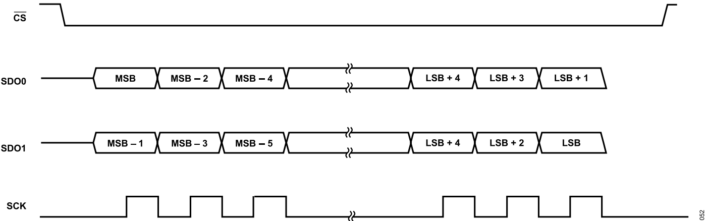
Figure 52. 2-Lane Mode, SDR Timing Diagram
