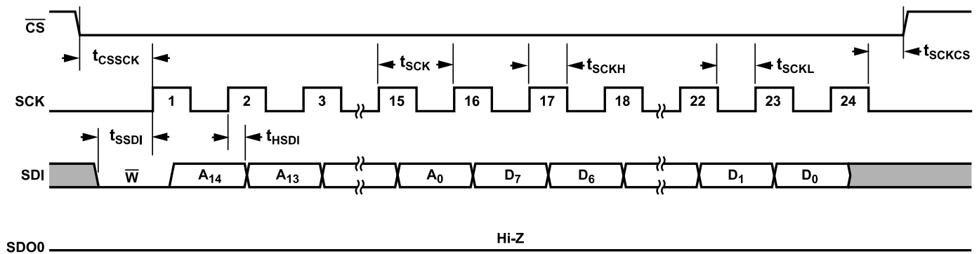
Figure 3. Register Configuration Mode Write Timing
