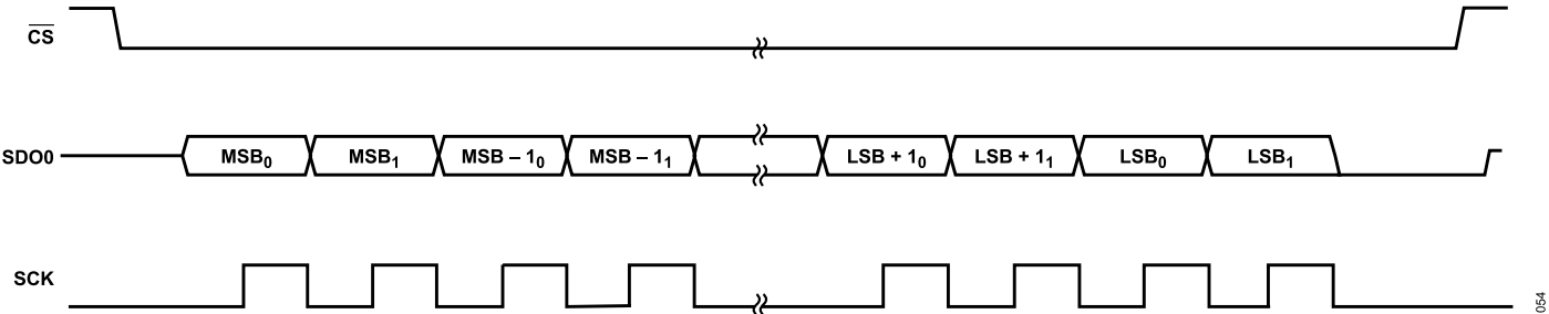
Figure 54. Interleaved Mode, SDR Timing Diagram
