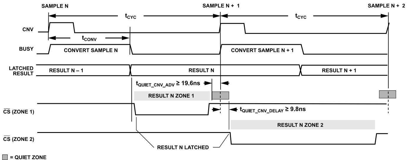
Figure 46. Example Timing for Data Transfer Zones
