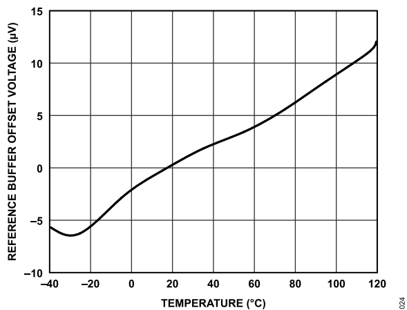
Figure 24. Reference Buffer Offset Voltage vs. Temperature
