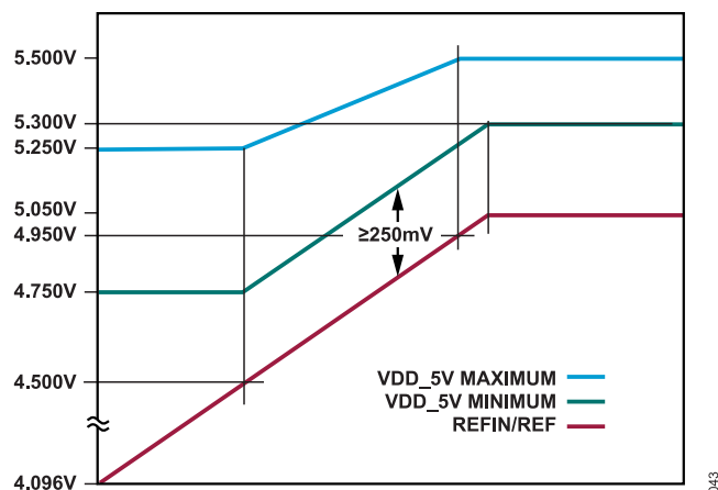
Figure 43. \text{VDD\_5V} Minimum and Maximum Values for \text{REFIN/REF}
