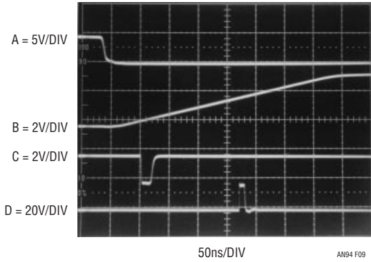
Figure 9. Pulse Generator's Waveforms Include Clock (Trace A), Q2's Collector Ramp (Trace B), Trigger Output (Trace C) and Pulse Output (Trace D). Delay Sets Output Pulse \approx 170ns After Trigger Output
