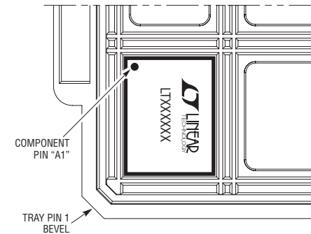
PACKAGE IN TRAY LOADING ORIENTATION
