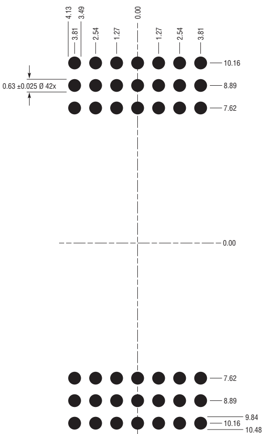
SUGGESTED PCB LAYOUT TOP VIEW
