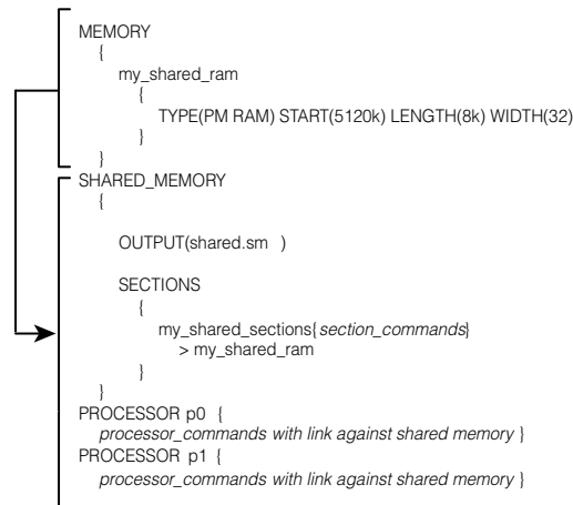
Figure 5-11: LDF Scopes for SHARED_MEMORY{ }
