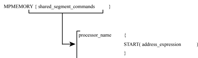
Figure 5-9: MPMEMORY{ } Command Syntax Tree
