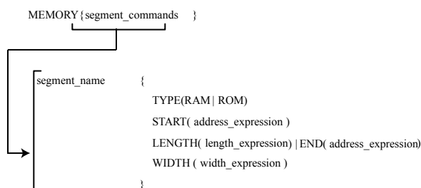
Figure 4-2: MEMORY{} Command Syntax Tree
