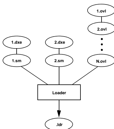
Figure 2-4: Input Files for a Multiprocessor System
