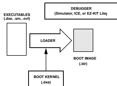
Figure 2-3: Using Loader to Create an Output File
