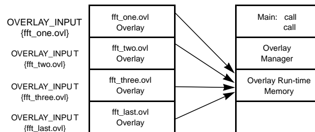
Figure 5-6: Example of Overlays - Not Grouped
