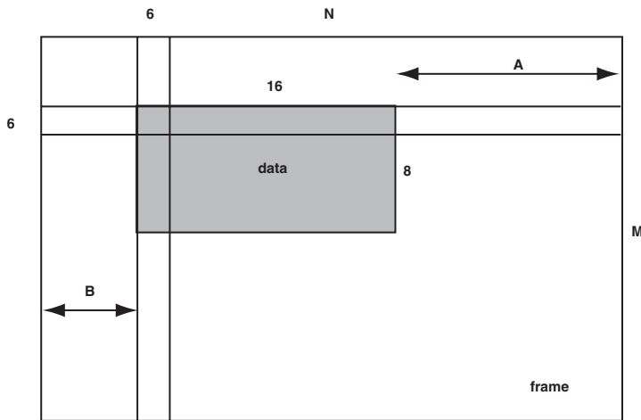
Figure 6-4. Selecting a 16 x 8 Block of Data from a Video Frame of Size N x M
