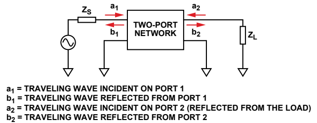
Figure 2. S-parameter model.
