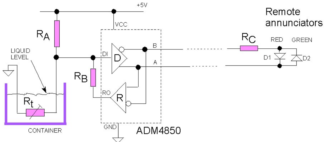
Figure 1. Thermistor senses when liquid is above or below a preset threshold.
